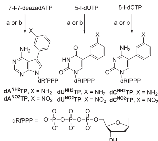
Scheme 1. Reagents and conditions: 3-aminophenylboronic acid (a) or 3-nitrophenylboronic acid (b) and \text{Cs}_2\text{CO}_3 , \text{Pd}(\text{OAc})_2 , \text{P}(\text{C}_6\text{H}_4-3-\text{SO}_3\text{Na})_3 , \text{H}_2\text{O}/\text{CH}_3\text{CN} (2:1).
